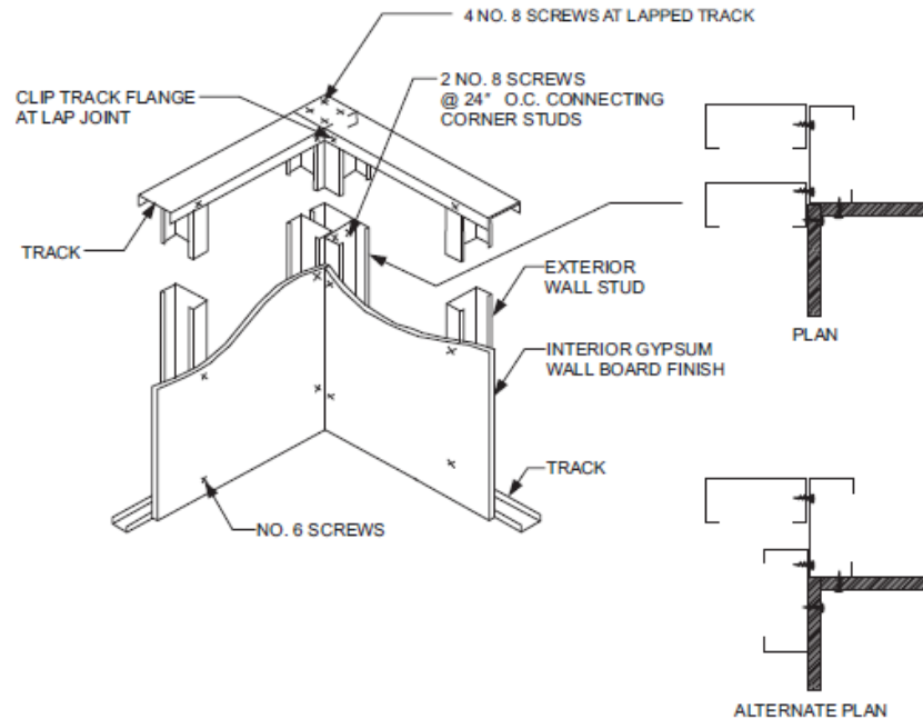
FIGURE 603.4 CORNER FRAMING
