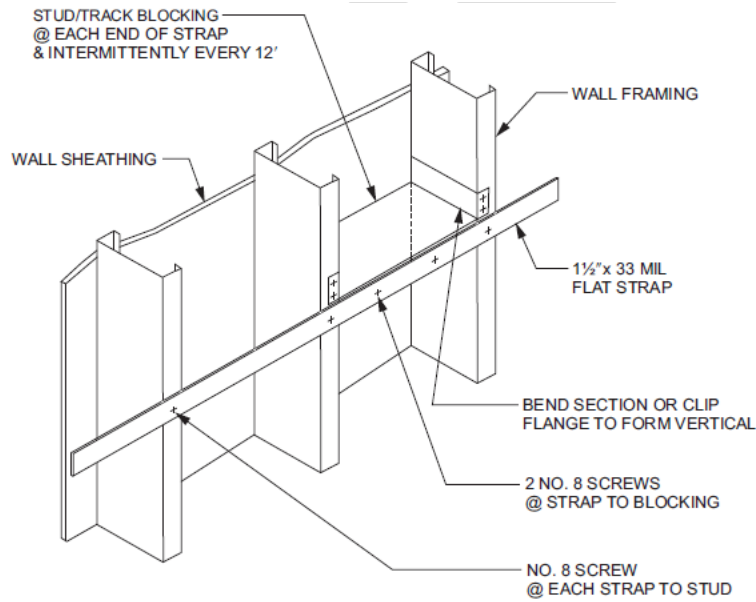
FIGURE 603.3.3(2) STUD BRACING WITH STRAPPING AND SHEATHING MATERIAL
