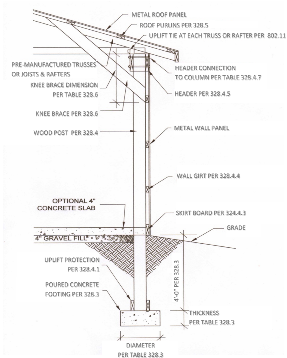
FIGURE 328 POST AND FRAME WALL SECTION. (NO SCALE)
