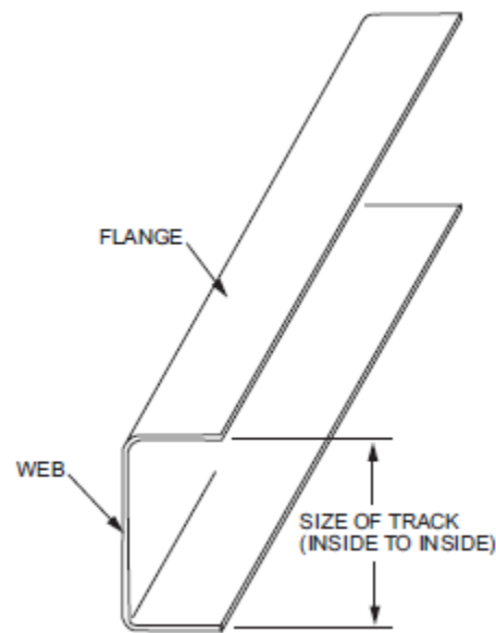
FIGURE 603.2.3(2) TRACK SECTION
