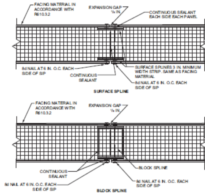
FIGURE 610.8 TYPICAL SIP WALL PANEL-TO-PANEL CONNECTION DETAILS
