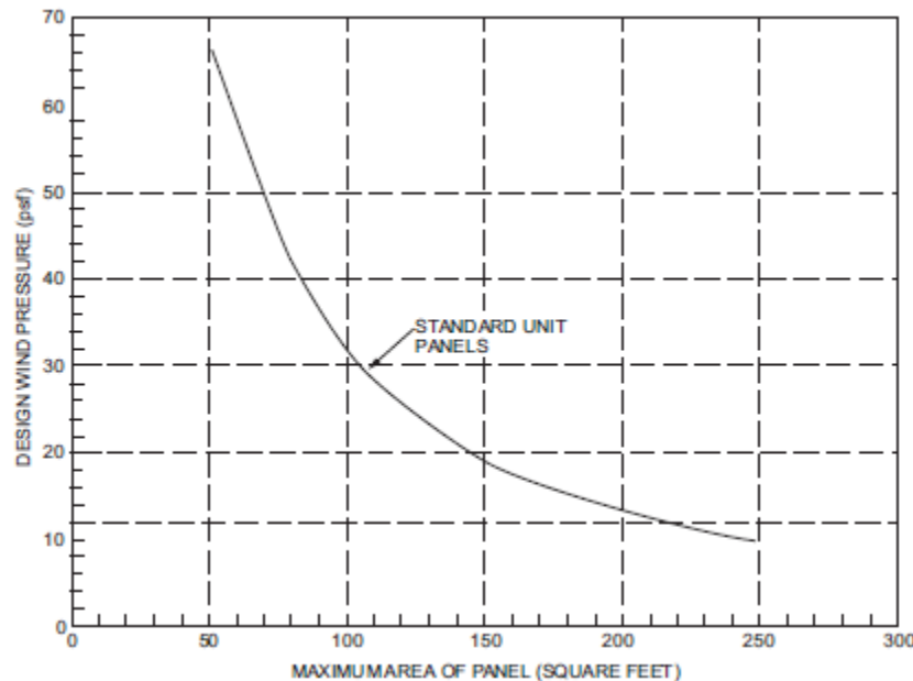
FIGURE 607.4.1 GLASS UNIT MASONRY DESIGN WIND LOAD RESISTANCE
