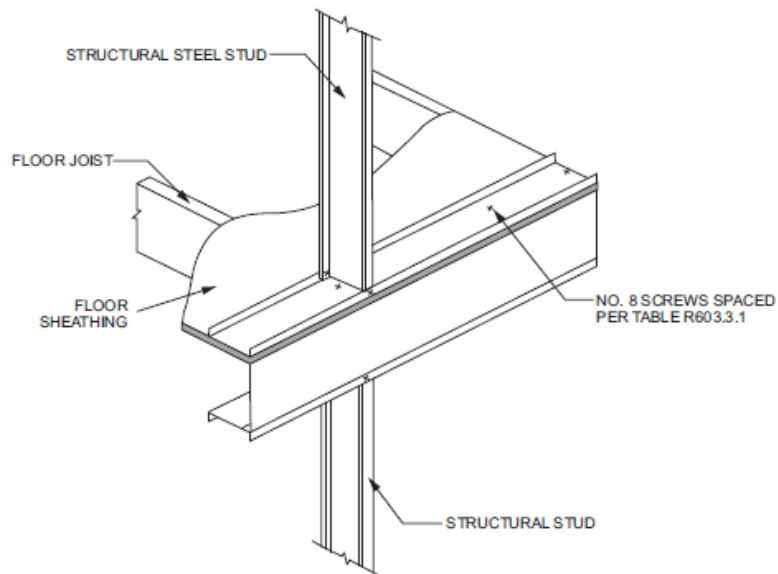
FIGURE 603.3.1(1) WALL TO FLOOR CONNECTION
