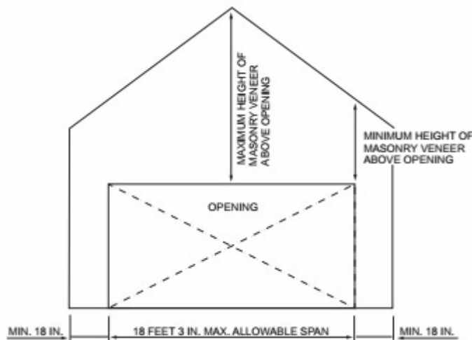
FIGURE 703.8.3.2 MASONRY VENEER OPENING
