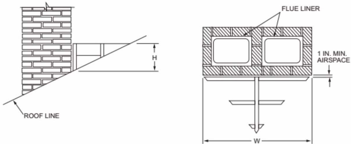
FIGURE 1003.20 CHIMNEY CRICKET
