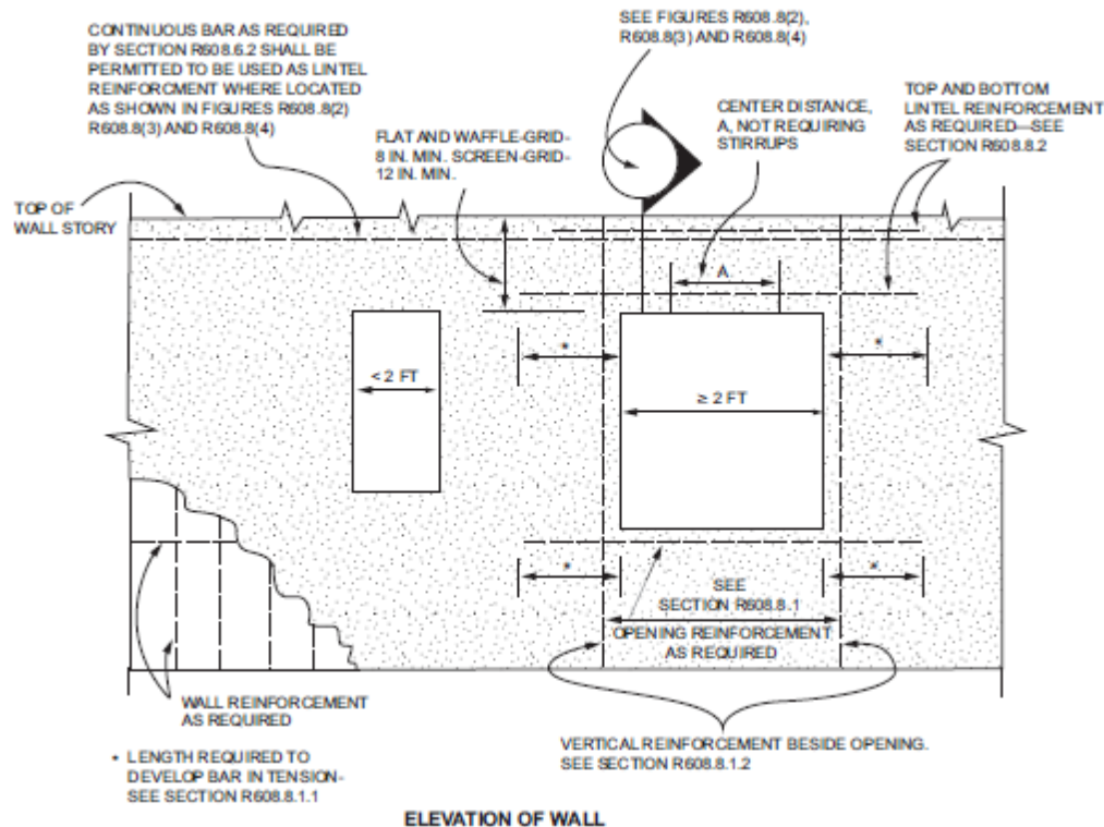
FIGURE 608.8(1) REINFORCEMENT OF OPENINGS
