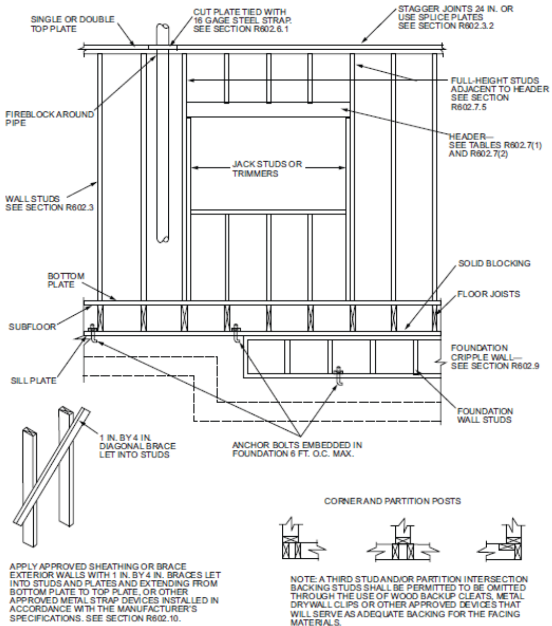
FIGURE 602.3(2) FRAMING DETAILS
