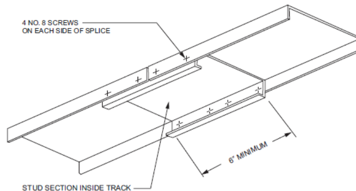
FIGURE 603.3.5 TRACK SPLICE
