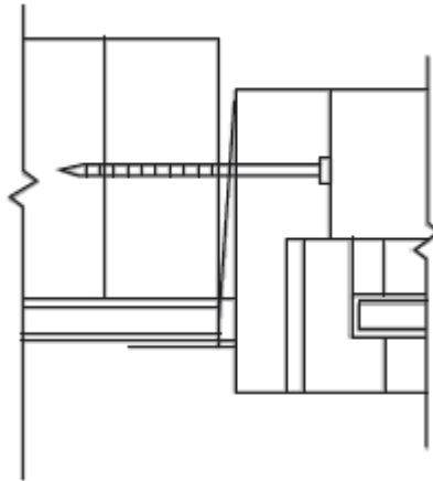
FIGURE 609.7.2(6) THROUGH THE FLANGE
