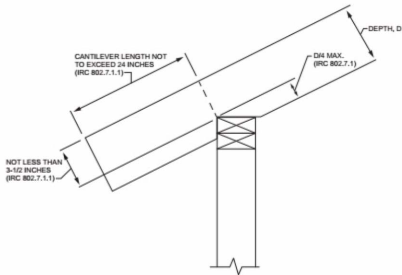
FIGURE 802.7.1.1 RAFTER NOTCH
