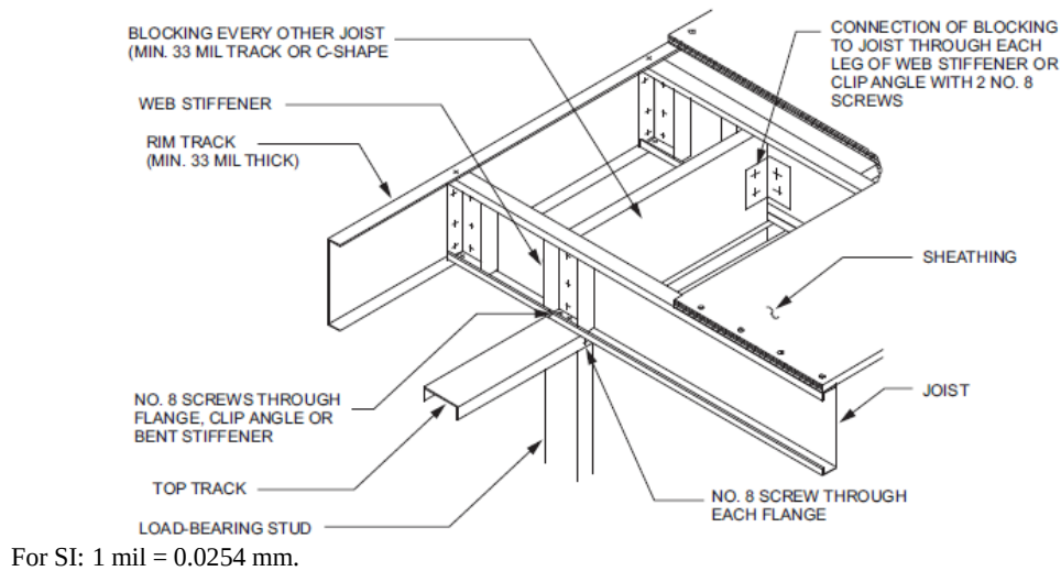
FIGURE 505.3.1(6) CANTILEVERED FLOOR TO EXTERIOR LOAD-BEARING WALL CONNECTION
