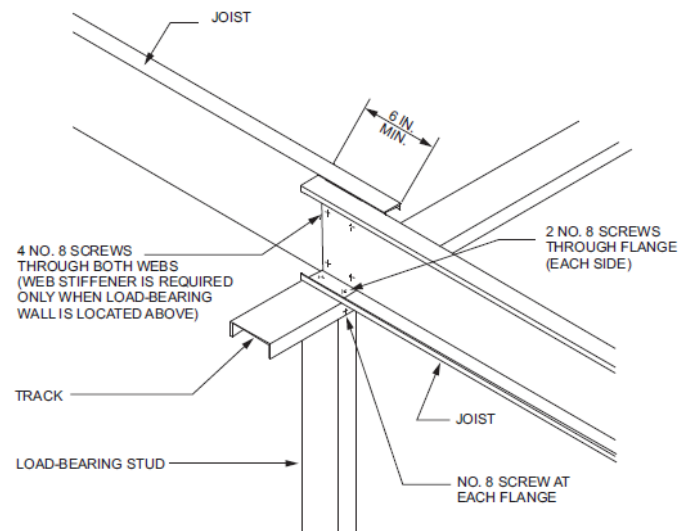
FIGURE 505.3.1(8) LAPPED JOISTS SUPPORTED ON INTERIOR LOAD-BEARING WALL
