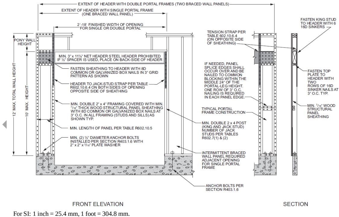
FIGURE 602.10.6.3 METHOD PFG—PORTAL FRAME AT GARAGE DOOR OPENINGS IN SEISMIC DESIGN CATEGORIES A, B and C
