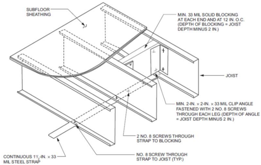
FIGURE 505.3.3.2(1) JOIST BLOCKING (SOLID)
