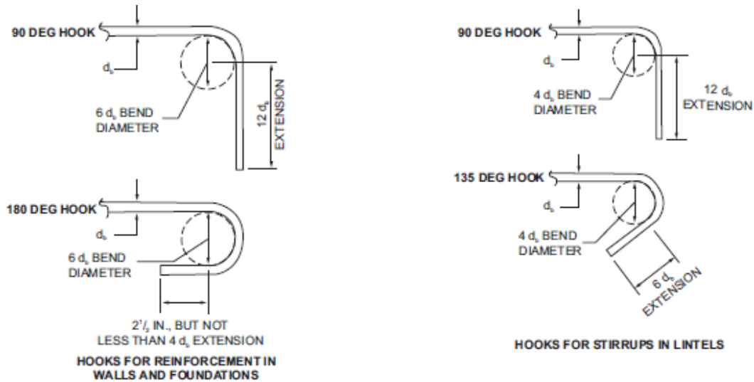
FIGURE 608.5.4(3) STANDARD HOOKS
