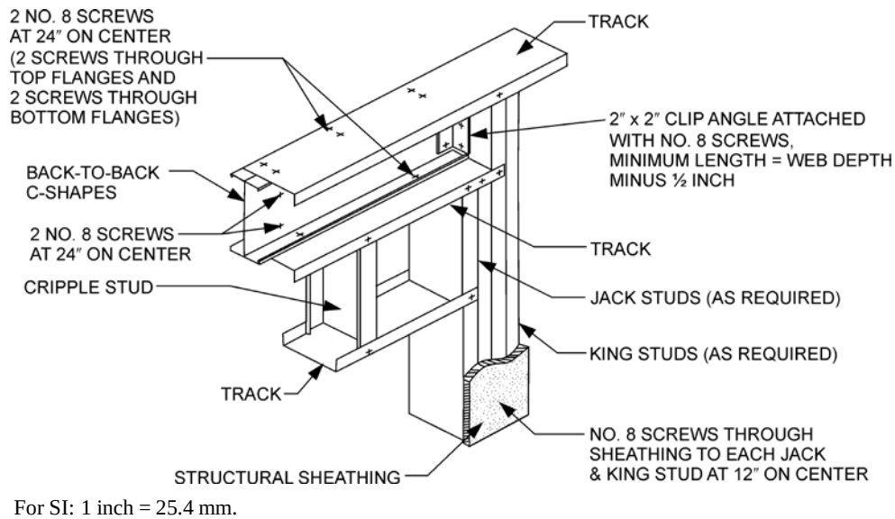
FIGURE 603.6(2) BACK-TO-BACK HEADER
